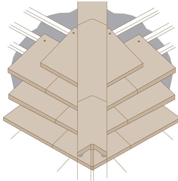
Capped hip
