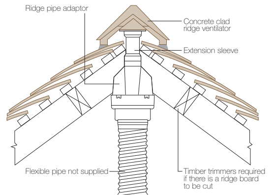
Ridge ventilator installed as soil vent or mechanical extract terminal (Installation required in unheated roof space)
