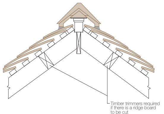
Ridge ventilator installed for roof space ventilation
