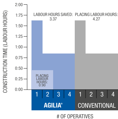
Placement* time of 1m 2 concrete
