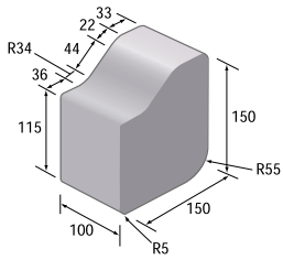
Main unit MK.
