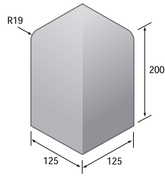
BN Upright external angle LK/G.
