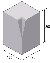
HB Upright internal angle LK/D.
