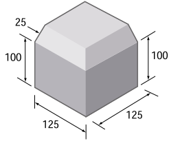
External angle SK/A.
