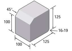
Crossing unit SK.
