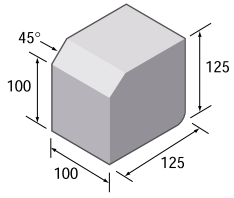
Main unit SK.
