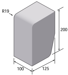
HB/BN Main unit LK.
