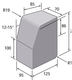
HB External radial block LK/C.
