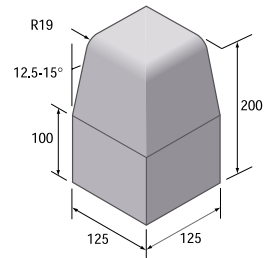
HB Upright external angle LK/E.
